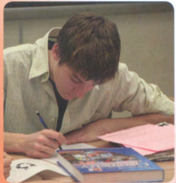
Jonathon Macoskey looks for a solution to the Konisburg Bridge problem. Because of the intensive proof work, logic was studied in the first semester .
